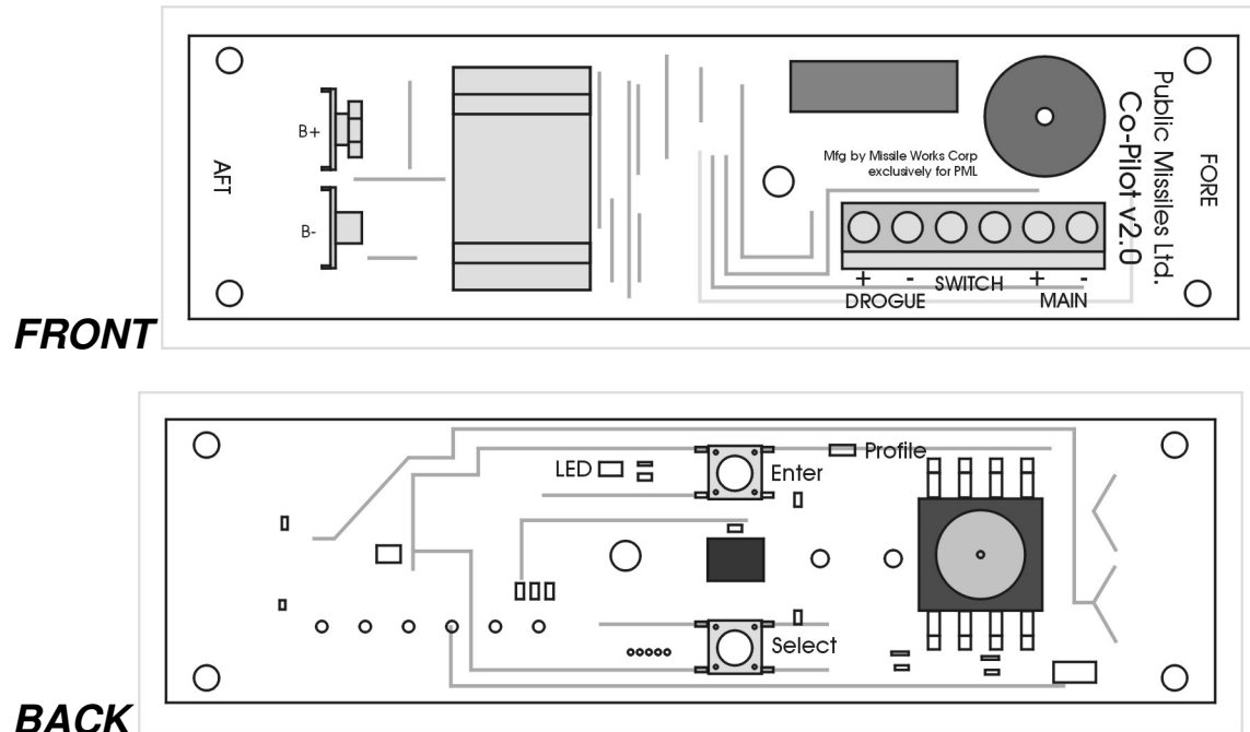
Figure 1 - Component Layout of the Co-Pilot v2.0
