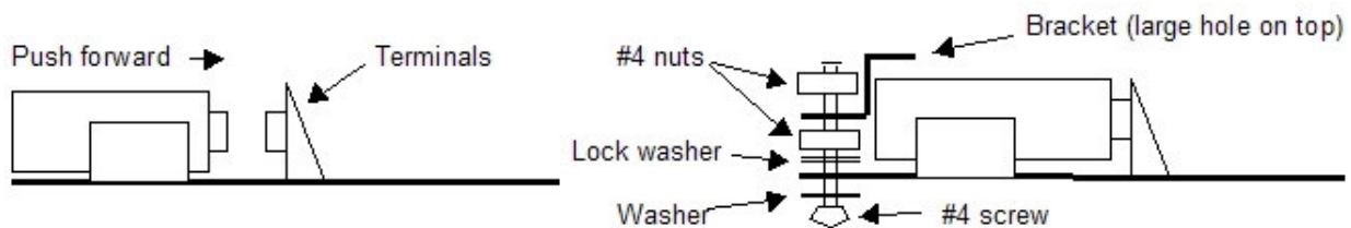
Figure 3 - Battery Retention Clip Detail
