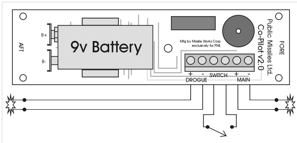
Figure 2 - Standard Wiring &amp; Connections
